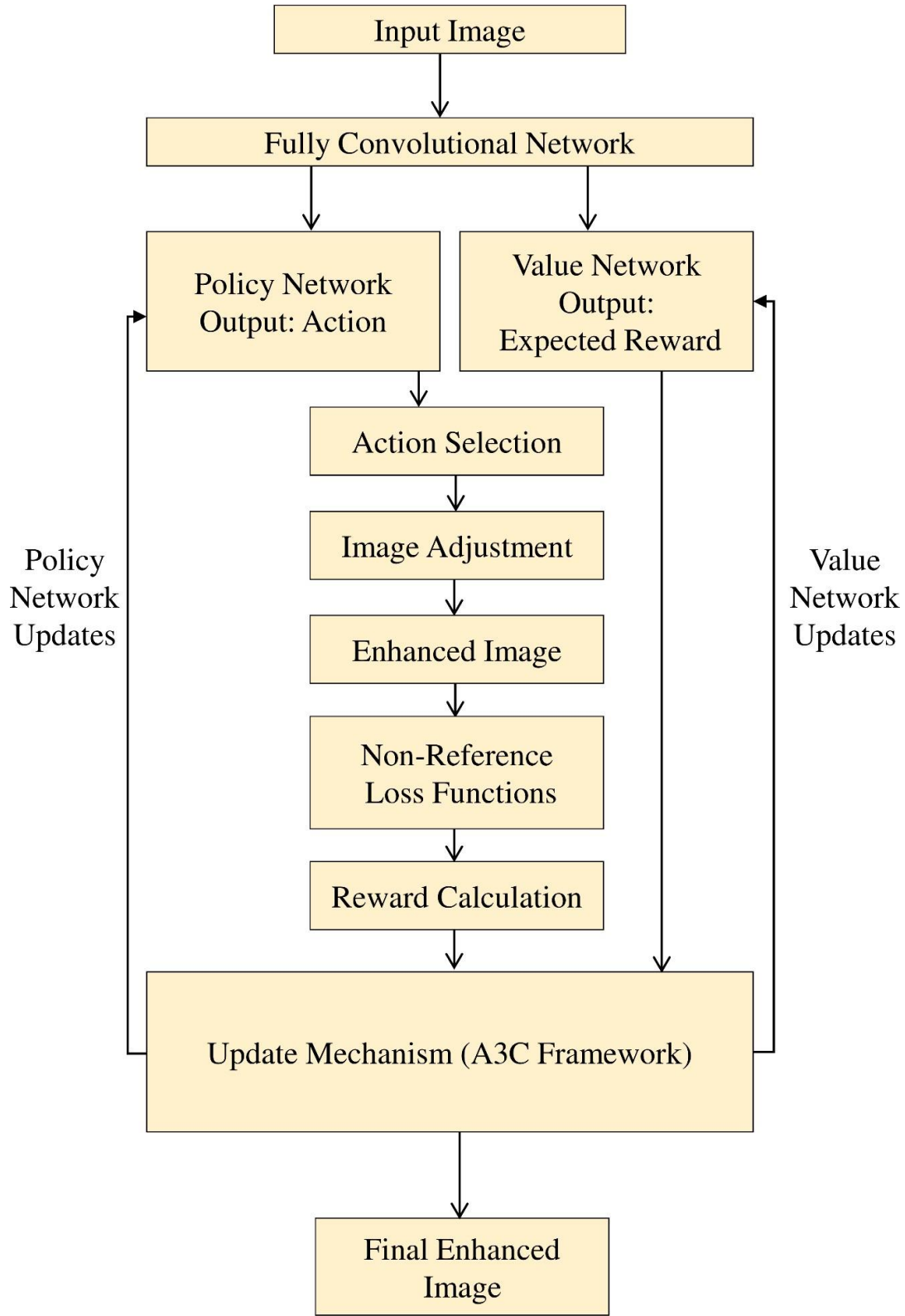
Figure (2): general diagram for the proposed reinforcement learning agent.
