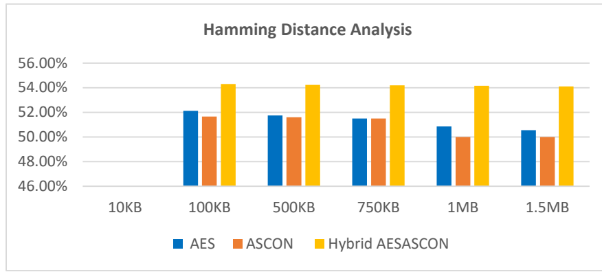
Figure7. Hamming distance analysis results of the proposed AESASCON method.
