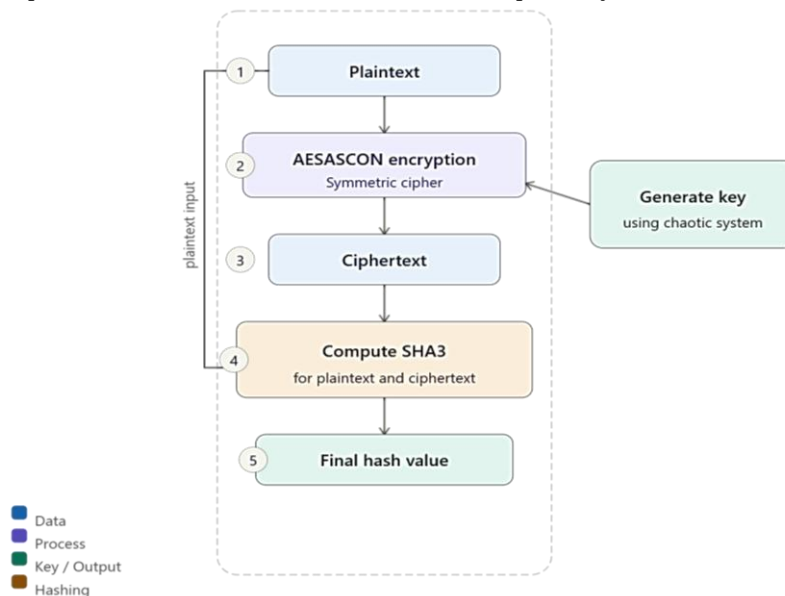
Figure3. Block diagram for computing hash value H1 at the sender's side
