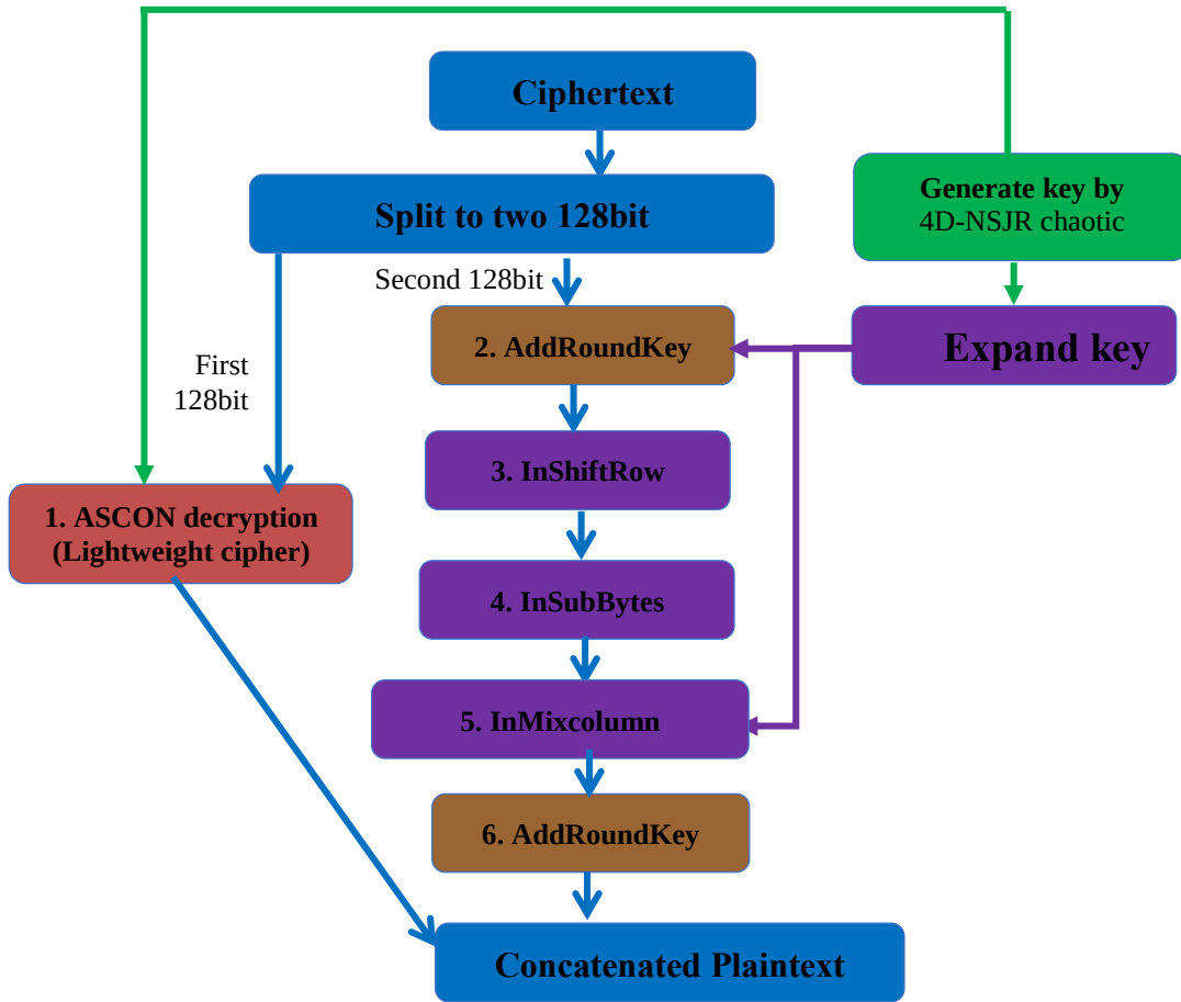
Figure2. Block diagram of the AESASCON decryption process.
