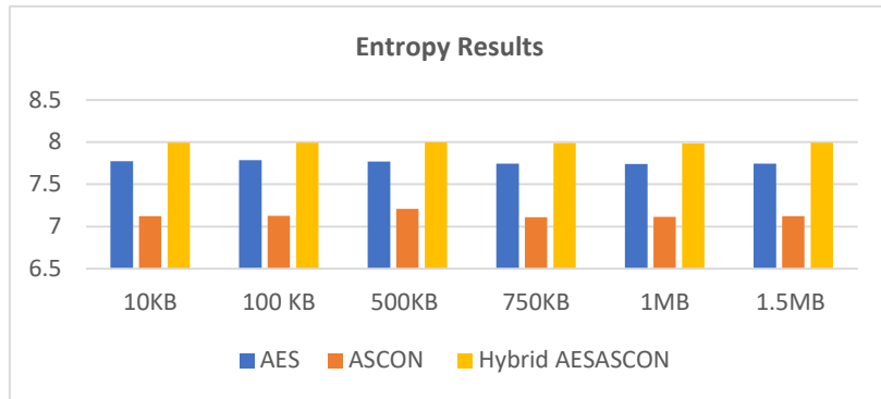
Figure 9. Entropy results of the proposed AESASCON method.
