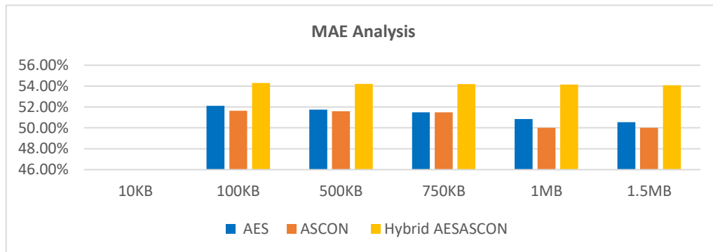
Figure 8. Mean absolute error results of the proposed AESASCON method.
