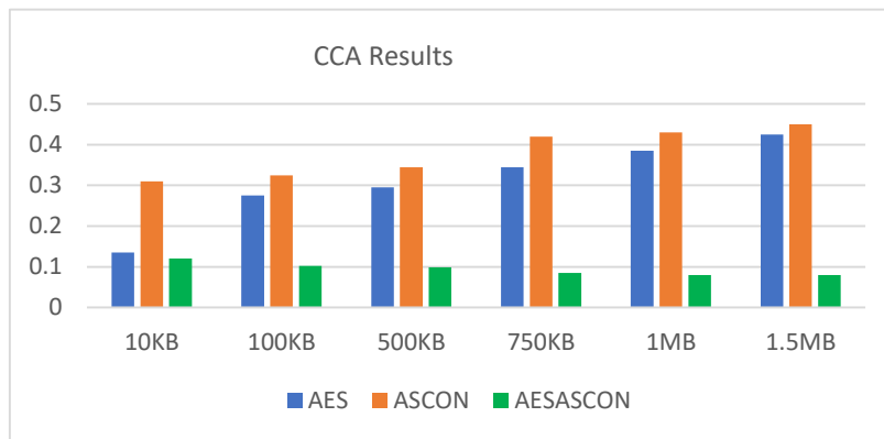
Figure 6. Correlation coefficient analysis results for the proposed AESASCON method.
