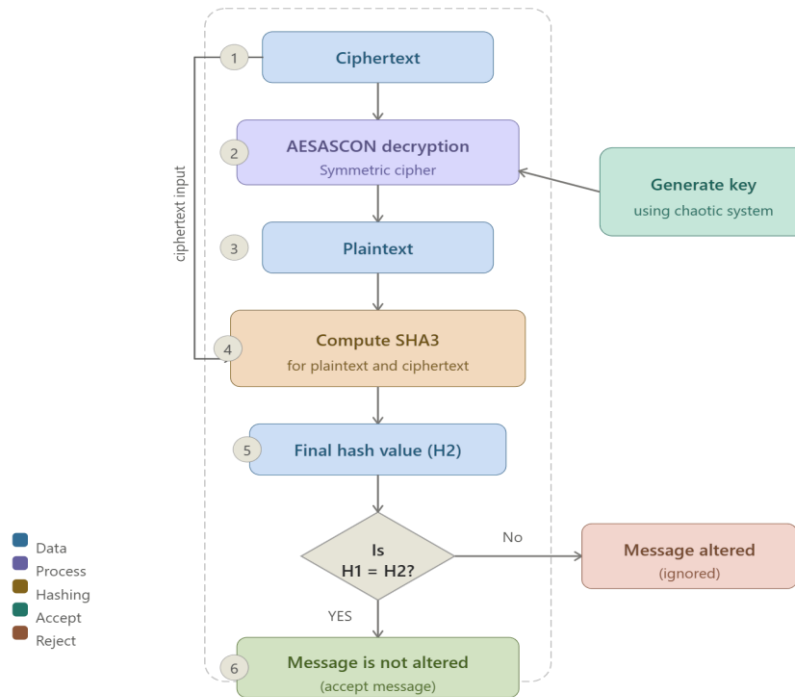
Figure4. Block diagram for computing hash value H2 at the receiver's side.
